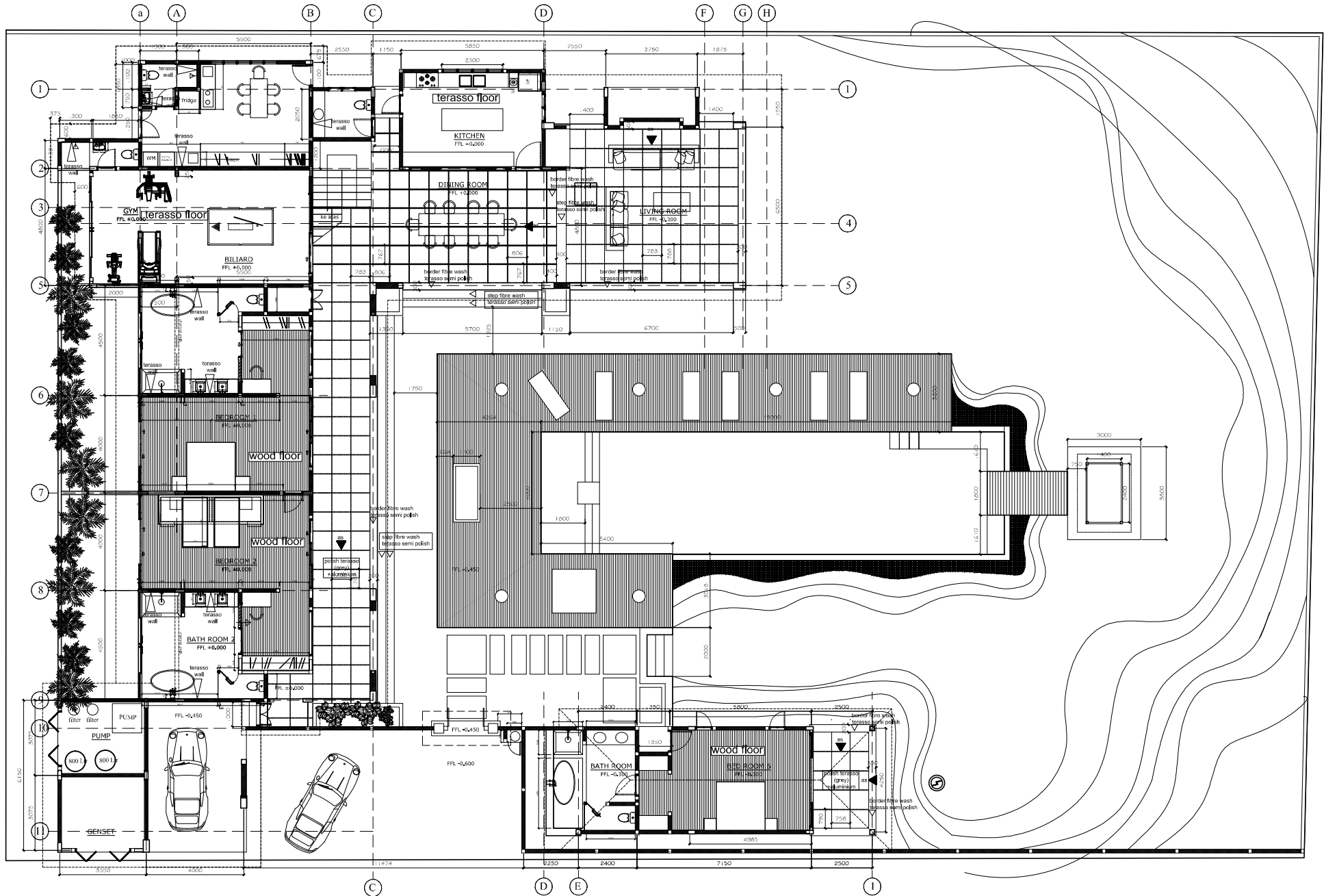
FINISHING PLAN GROUND FLOOR SCALE 1:150
