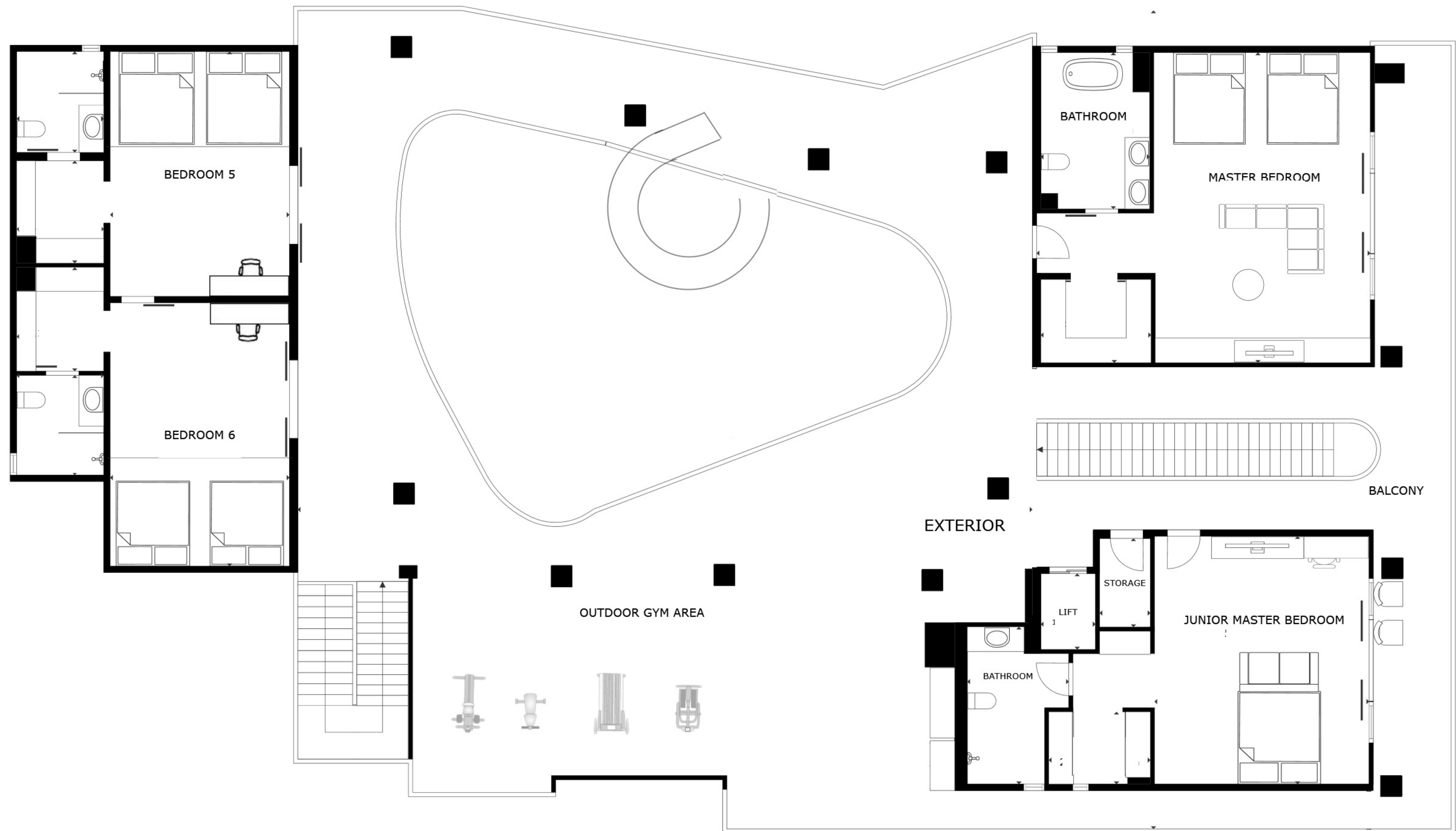
UPPER LEVEL
